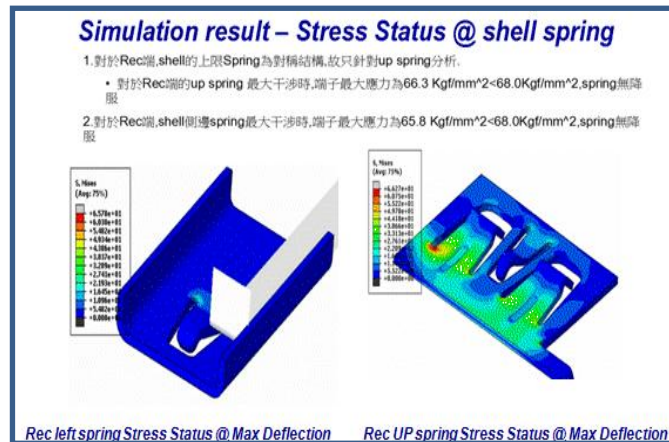
Part Design simulation
