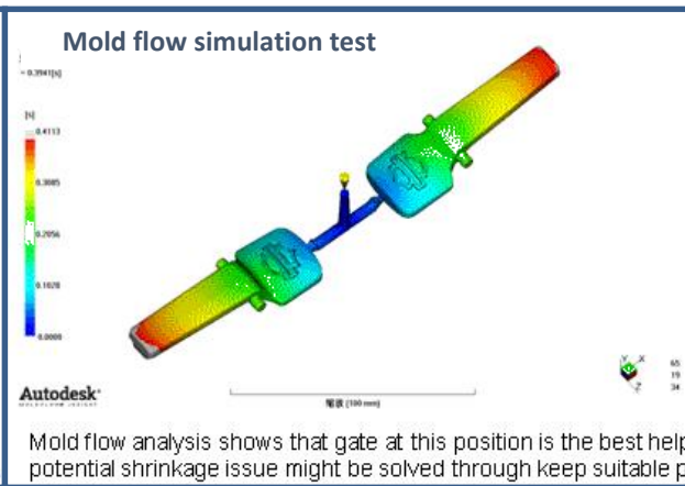
Tooling design simulation
