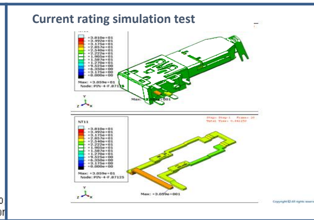
Rating test simulation
